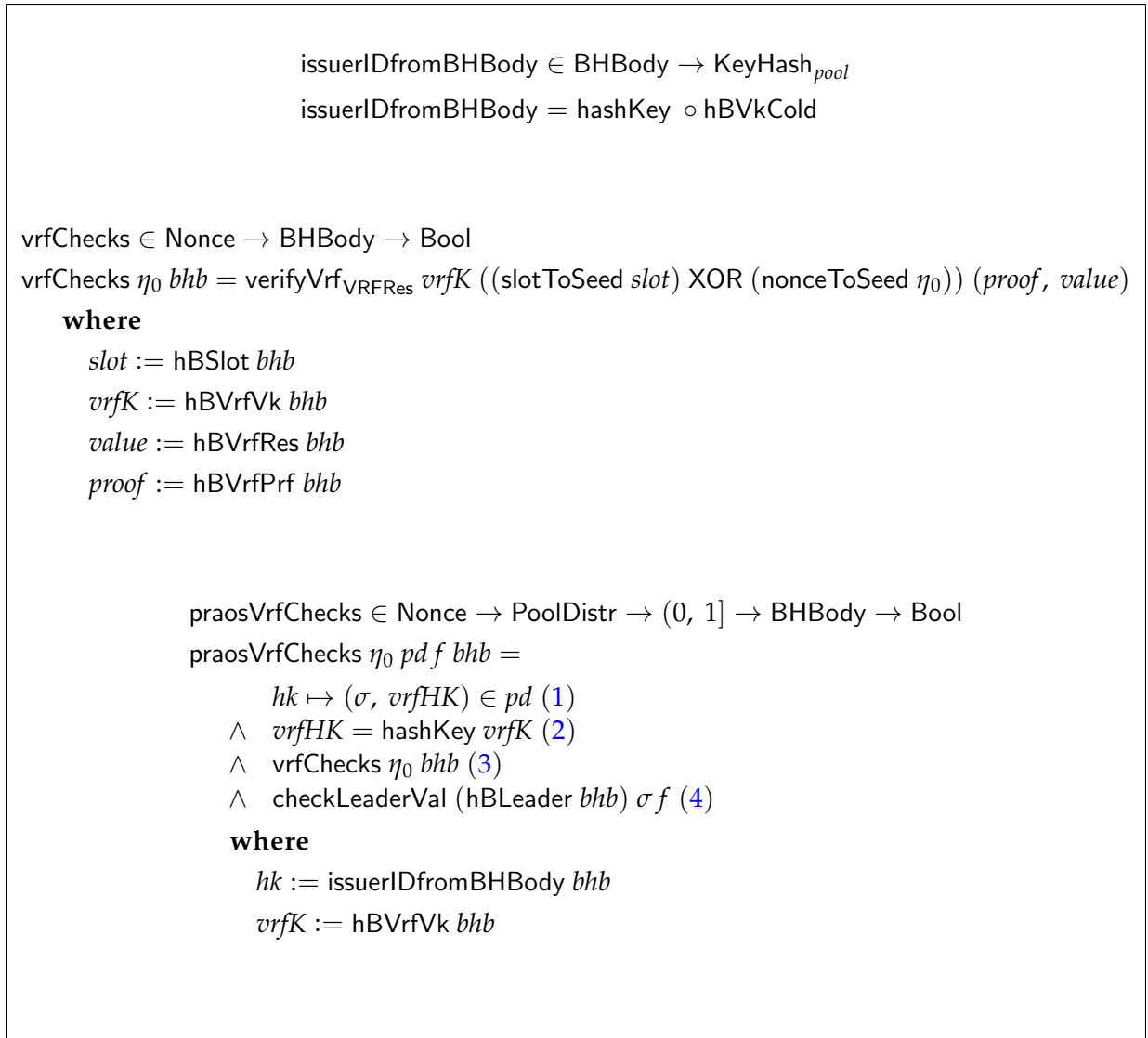
Figure 11: VRF helper functions
